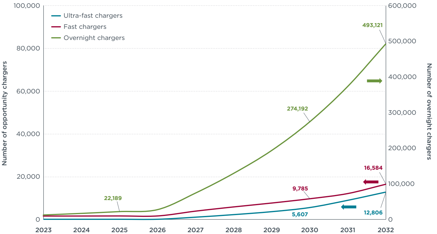
Figure 5. Cumulative U.S. EV medium- and heavy-duty charging needs, by charger type through 2032. Directional arrows indicate the corresponding axis.
